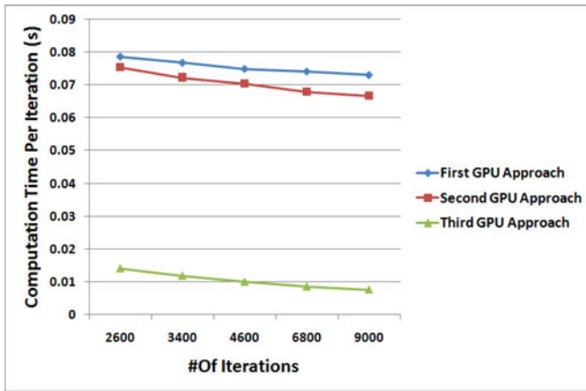
Fig. 7. Computation time per iteration of the three GPU approaches (456 floes).
