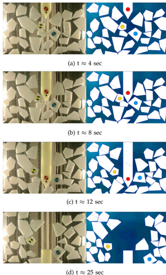
Fig. 20. Comparison between the numerical simulation and the experiments of a single case. The bodies in the numerical model are manually given coloured dots for convenience.
