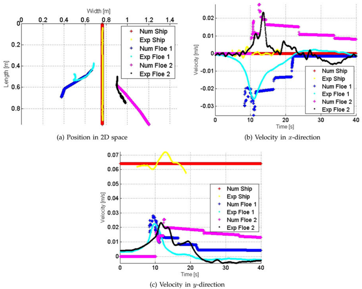
Fig. 19. Pack ice comparison, numerical model (Num) and experimental data (Exp).
