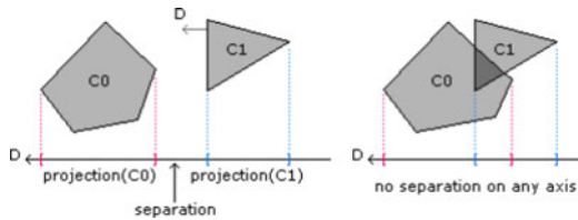
Fig. 5. Nonintersecting convex polygons (left). Intersecting convex polygons (right) [27].
