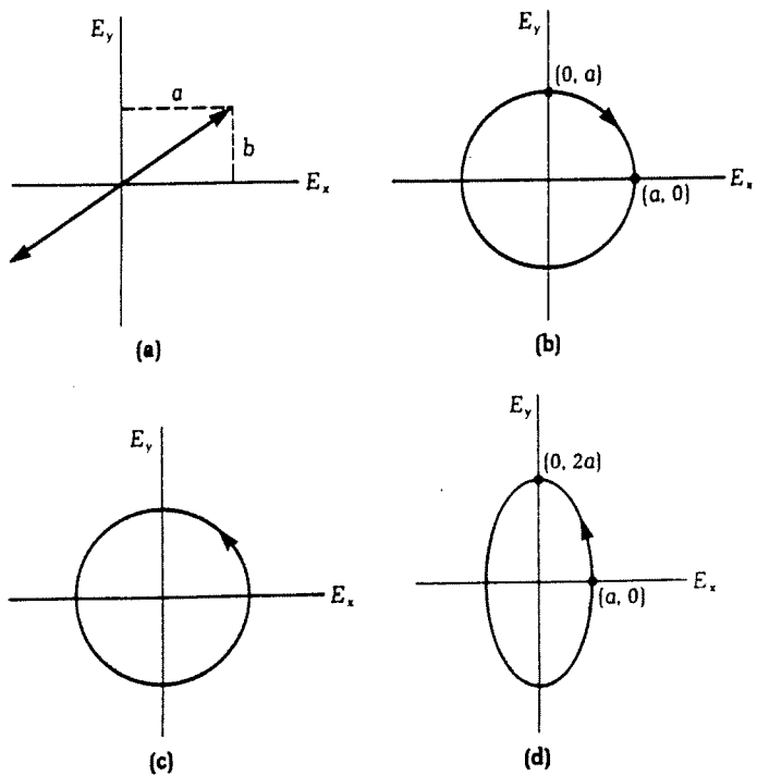
Polarization of an electric field: (a) Linear polarization. (b) Circular polarization (left-hand circular polarization if wave propagates in \hat{z} direction). (c) Circular polarization (right-hand if wave propagates in \hat{z} direction). (d) Elliptical polarization.
