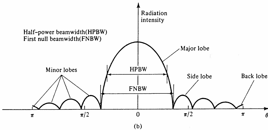
(a) Radiation lobes and beamwidths of an antenna pattern. (b) Linear plot of power pattern and its associated lobes and beamwidths.
