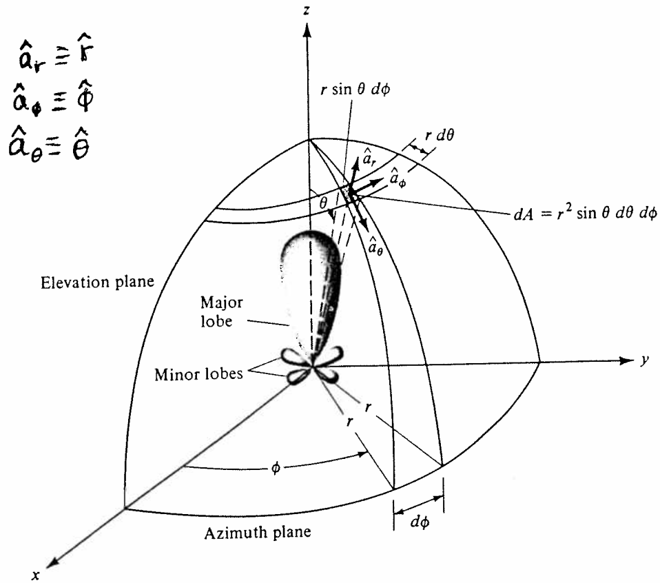
Coordinate system for antenna analysis.
